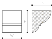
Corbel small
